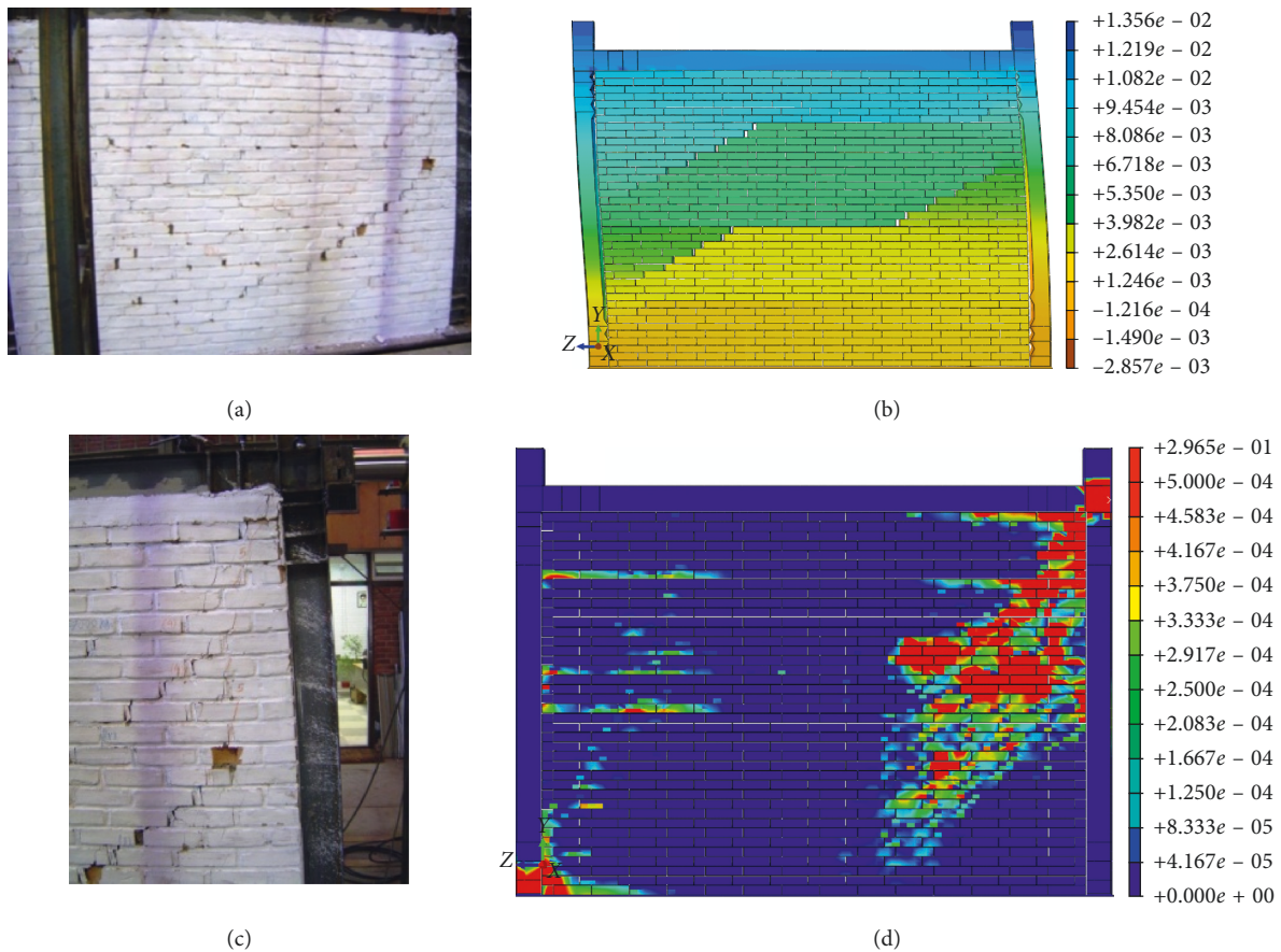
FIGURE 6: Comparison of the results between the experimental specimen and the numerical model. (a) Failure mode of the experimental specimen [24]. (b) Failure mode of the numerical model. (c) Crushing of bricks in the experimental specimen [24]. (d) Crushing of bricks in the numerical model.
